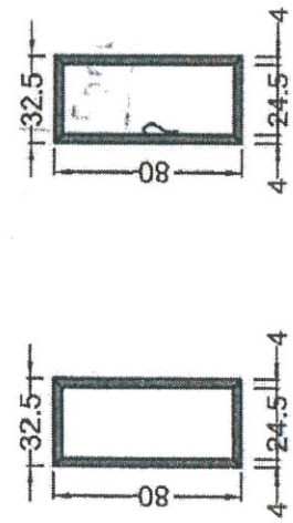
INNER FRAME OF WINDOW
